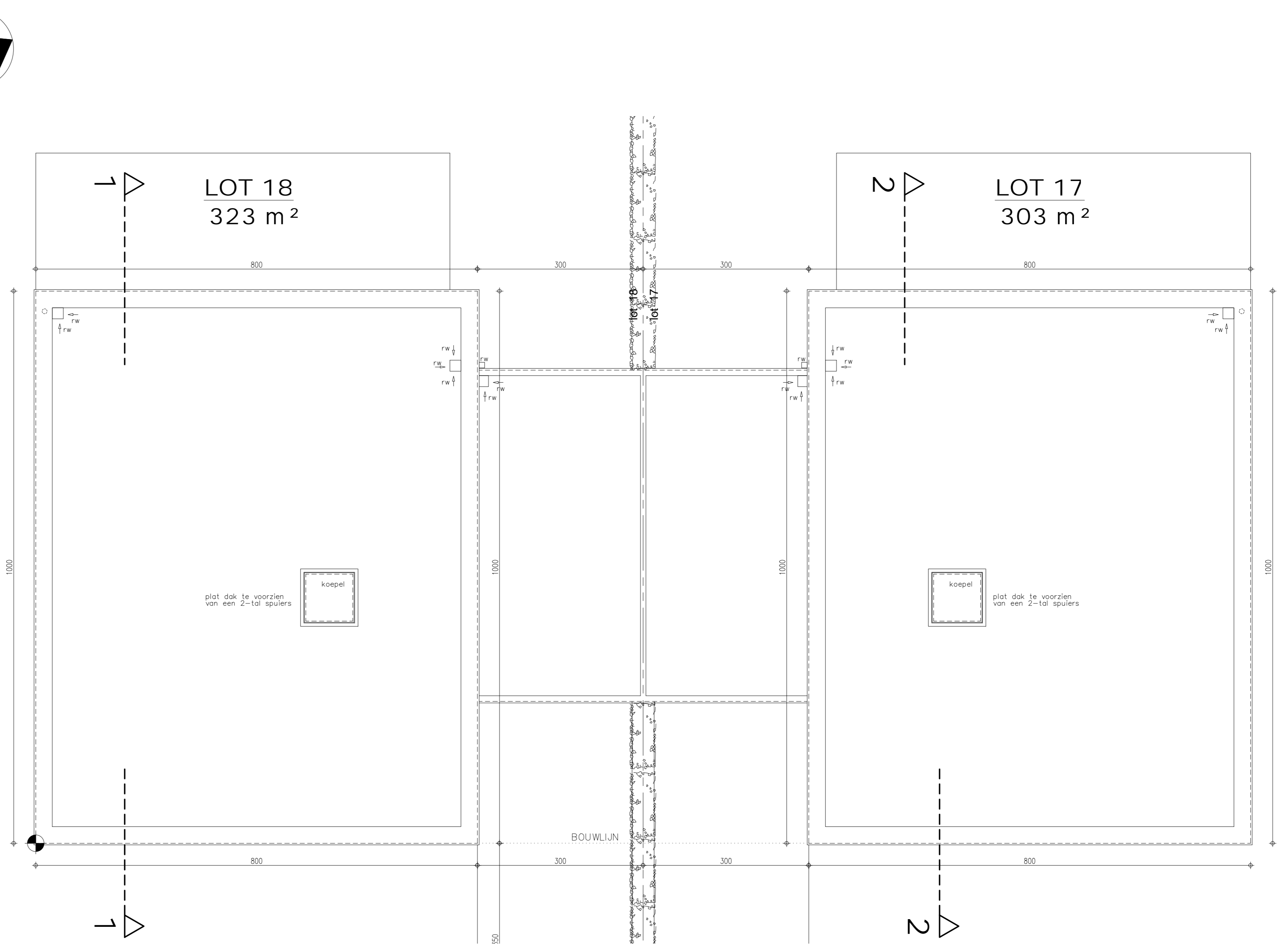
DAKENPLAN 1/50
