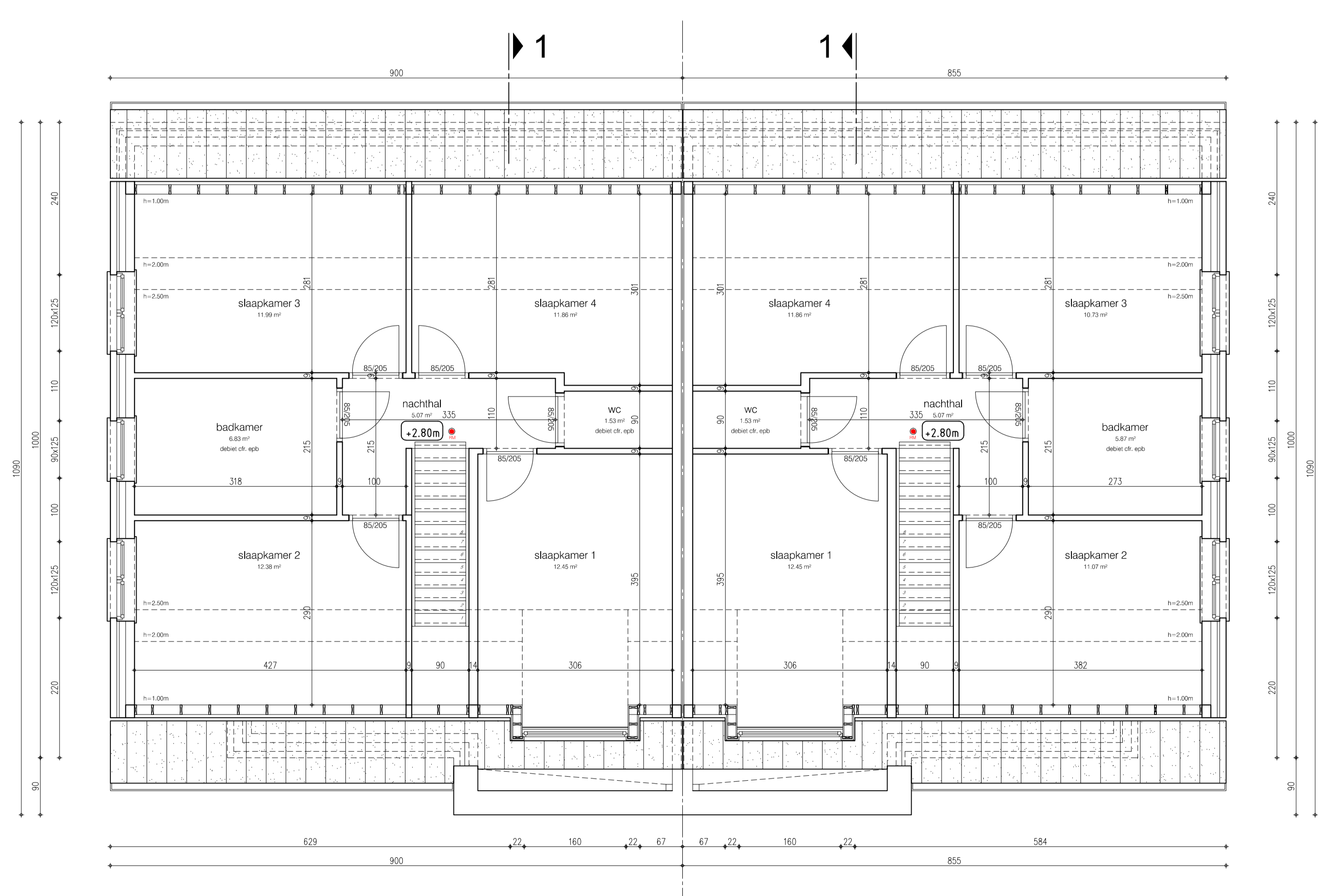
verdiepingsplan lot 28
